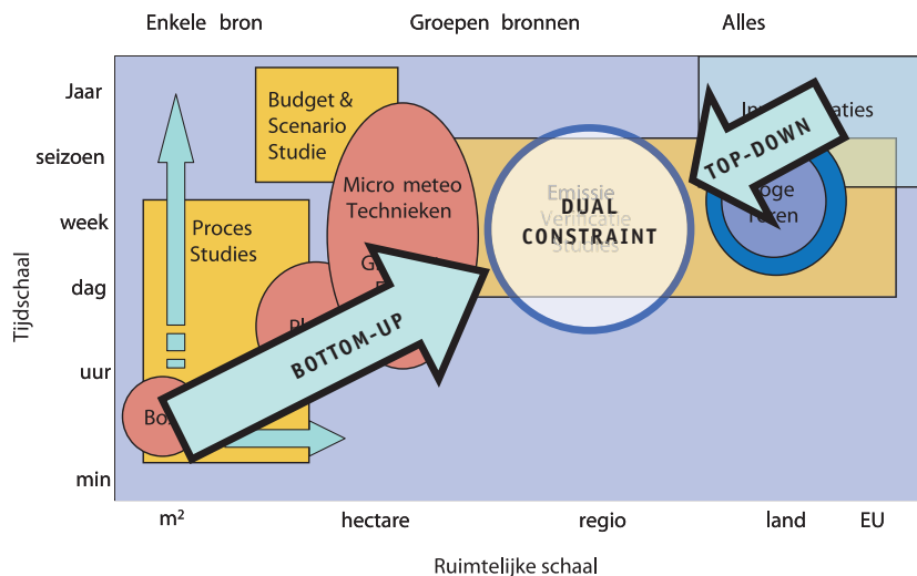
Figure 1 Through measurements on various scales in combination with down scaling techniques, the dual constraint method works from two sides towards an estimate of landscape emissions (based on figure 1 in Hensen et al., this issue).
